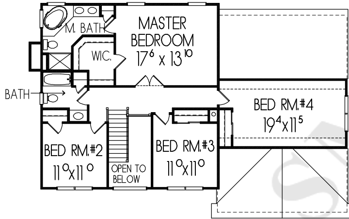
SECOND FLOOR PLAN 4-BEDROOM
